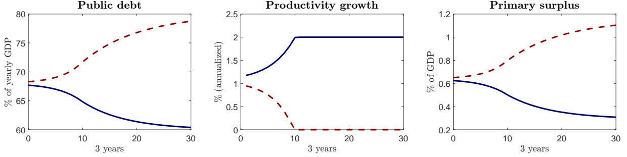
Figure 5: Fiscal hysteresis.
