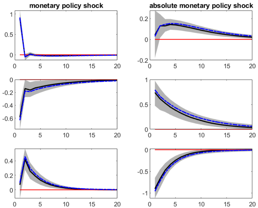
Figure A.1: Impulse response functions from the proxy-SVAR using 1000 data sets generated from (6) . Panel (a) simulation with standardized Normal structural shocks. Panel (b) the policy shock has a chi-square distribution with two degrees of freedom.
