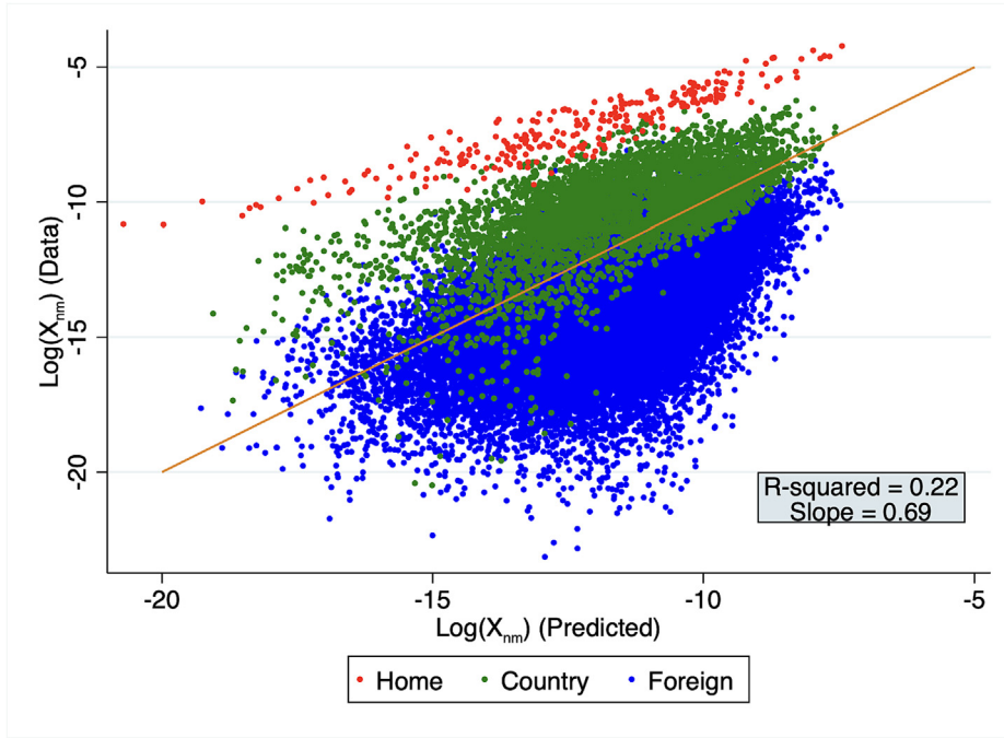
Fig. 4. Actual vs predicted trade (log) probabilities.
