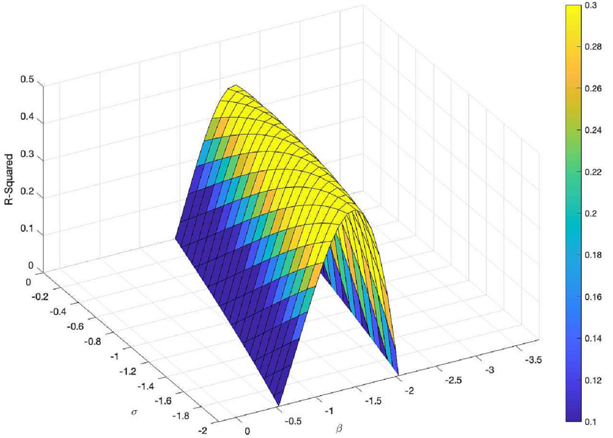
Fig. 12. Sensitivity analysis.
