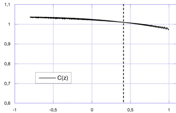
(f) Nominal debt: C(z) for \sigma = 1.4
