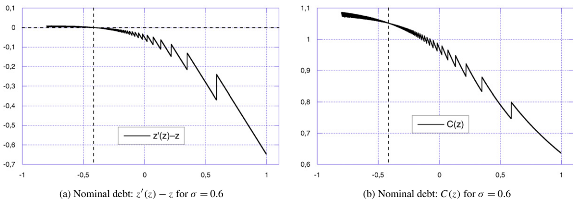
Fig. 2. Nominal debt for various values of \sigma .
