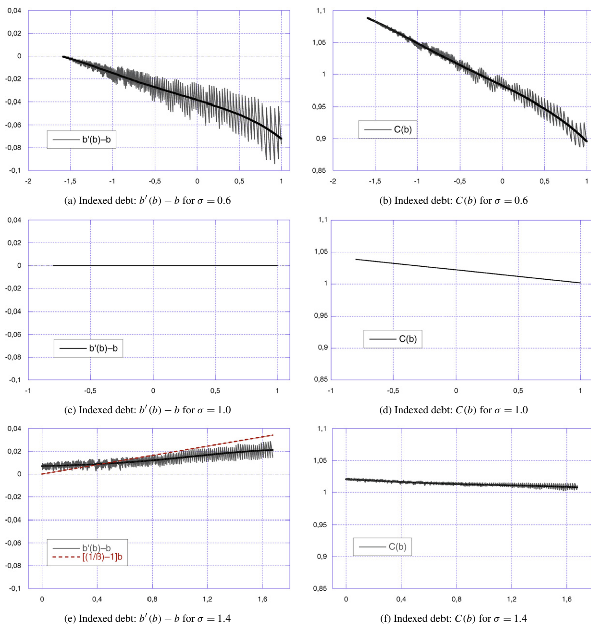
Fig. 1. Indexed debt for various values of \sigma .
