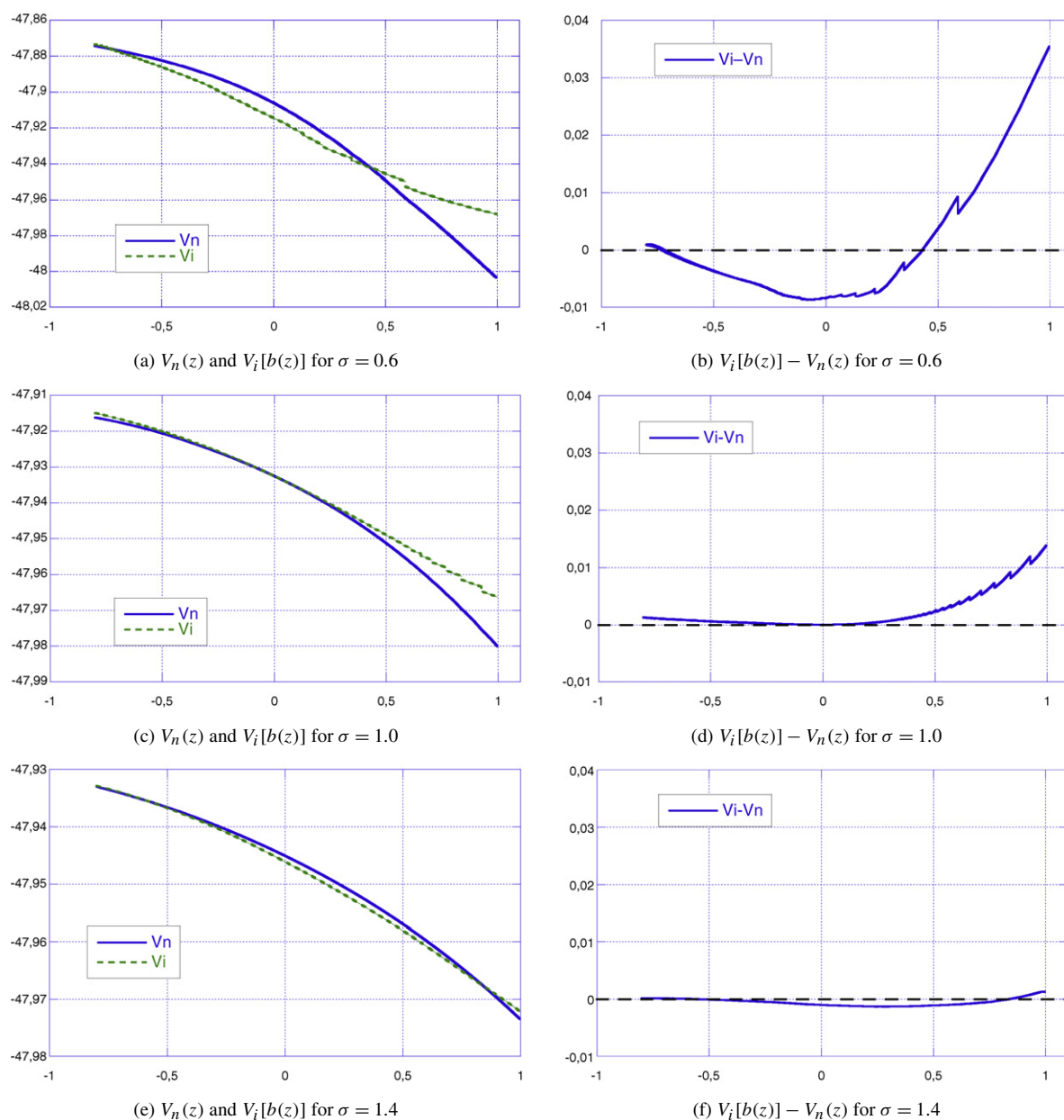
Fig. 4. Welfare comparisons for various values of \sigma .
