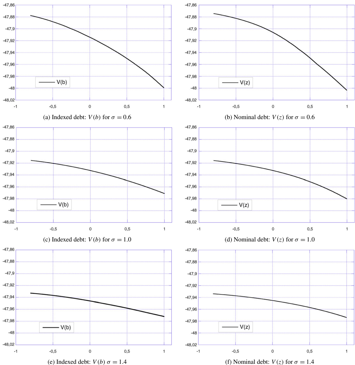
Fig. 3. Value functions for indexed and nominal debt and various values of \sigma .
