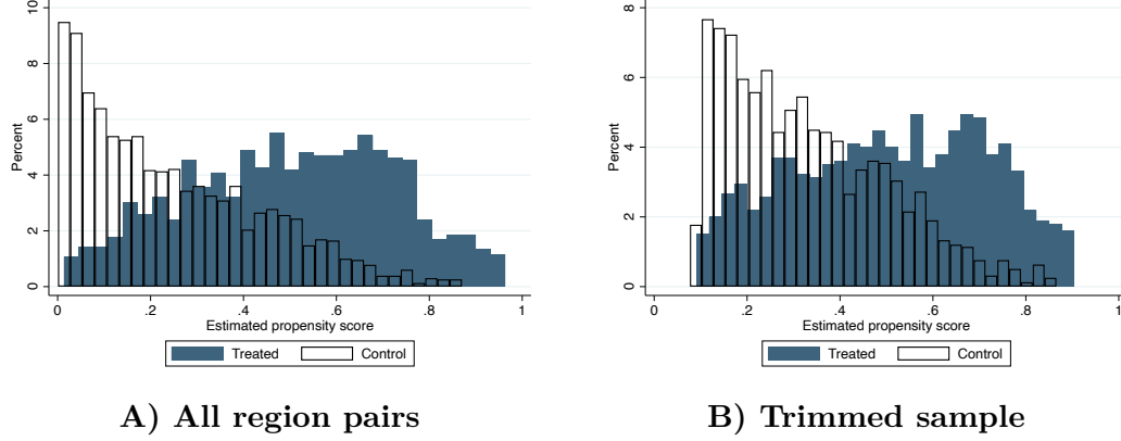
Figure 10: Histogram of propensity score
