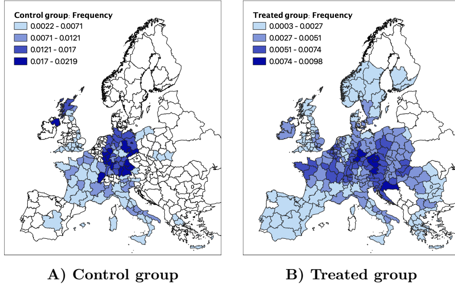
Figure A.15: Composition of regions in block 8
