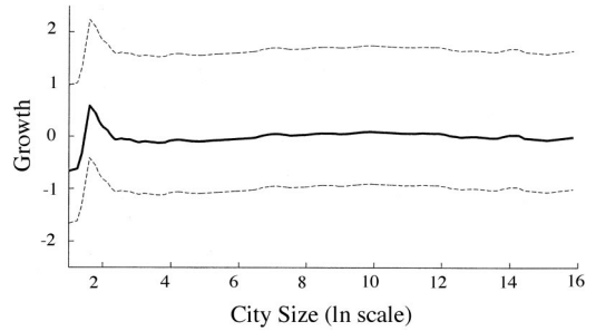
FIGURE 7. KERNEL ESTIMATE OF POPULATION GROWTH (BANDWIDTH 0.5)
