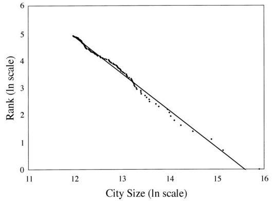
FIGURE 9. CITY SIZE DISTRIBUTION AND LINEAR REGRESSION LINE
