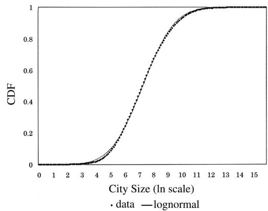
FIGURE 3. EMPIRICAL AND THEORETICAL CUMULATIVE DENSITY FUNCTIONS
