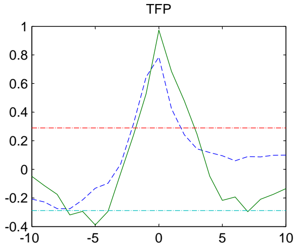
Figure 20: Cross correlation with output for data (dash) and model (solid).
